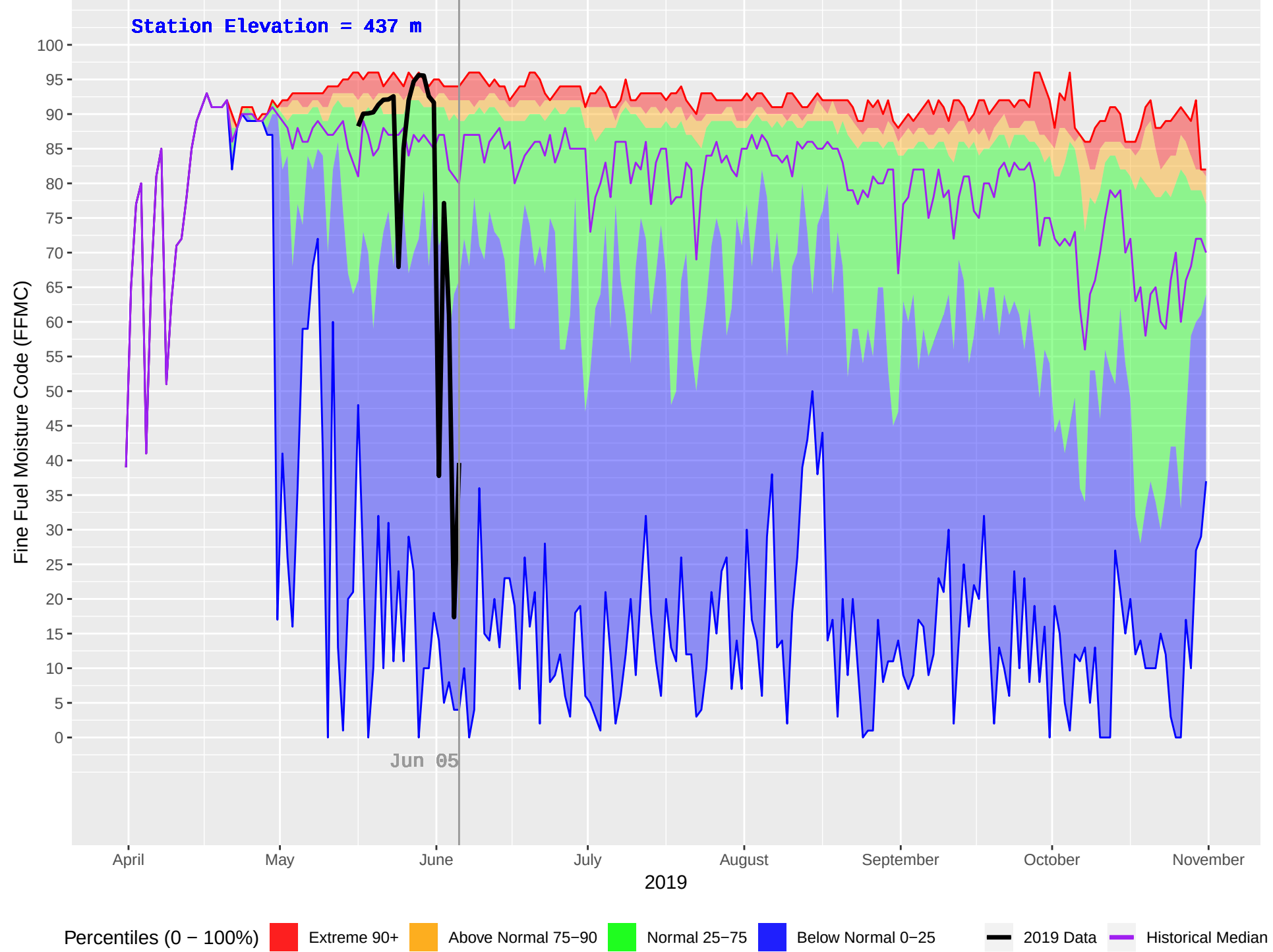
ELK MOUNTAIN (438) : Historical (1973–2018) and Current (2019) Daily Fine Fuel Moisture Code (FFMC)
