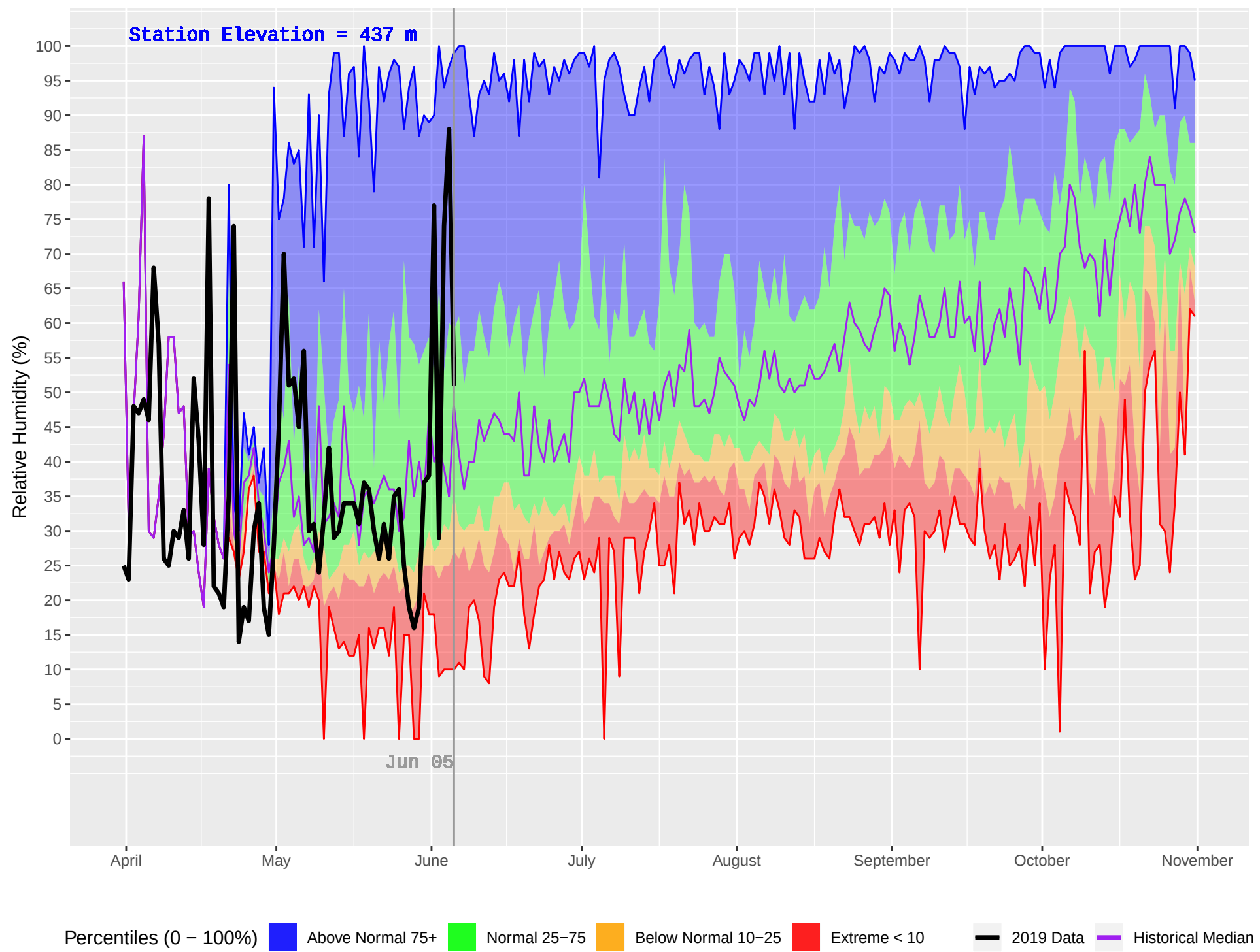
ELK MOUNTAIN (438) : Historical (1973–2018) and Current (2019) Daily Relative Humidity
