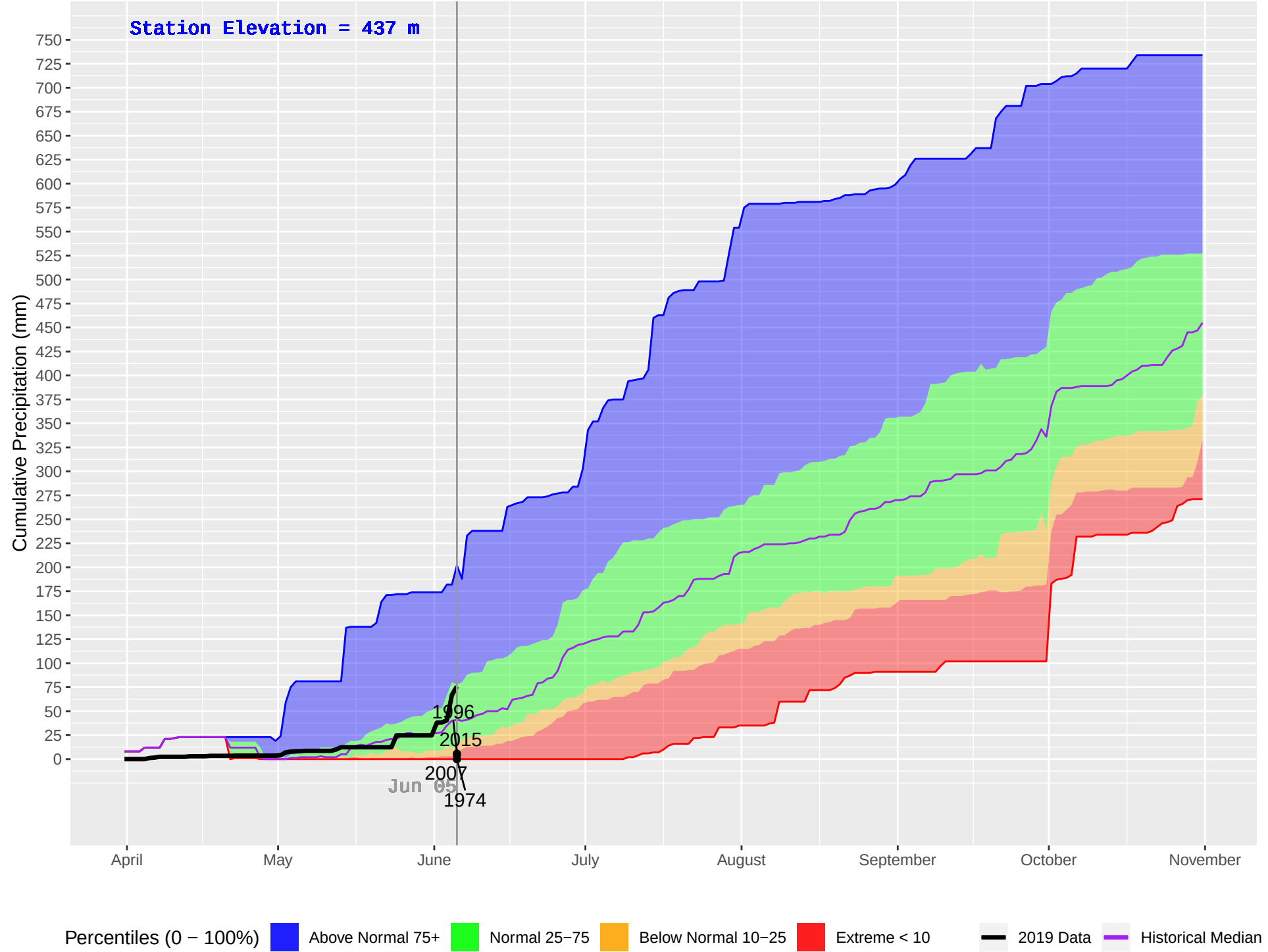
ELK MOUNTAIN (438) : Historical (1973–2018), Current (2019) Daily Cumulative Precipitation
