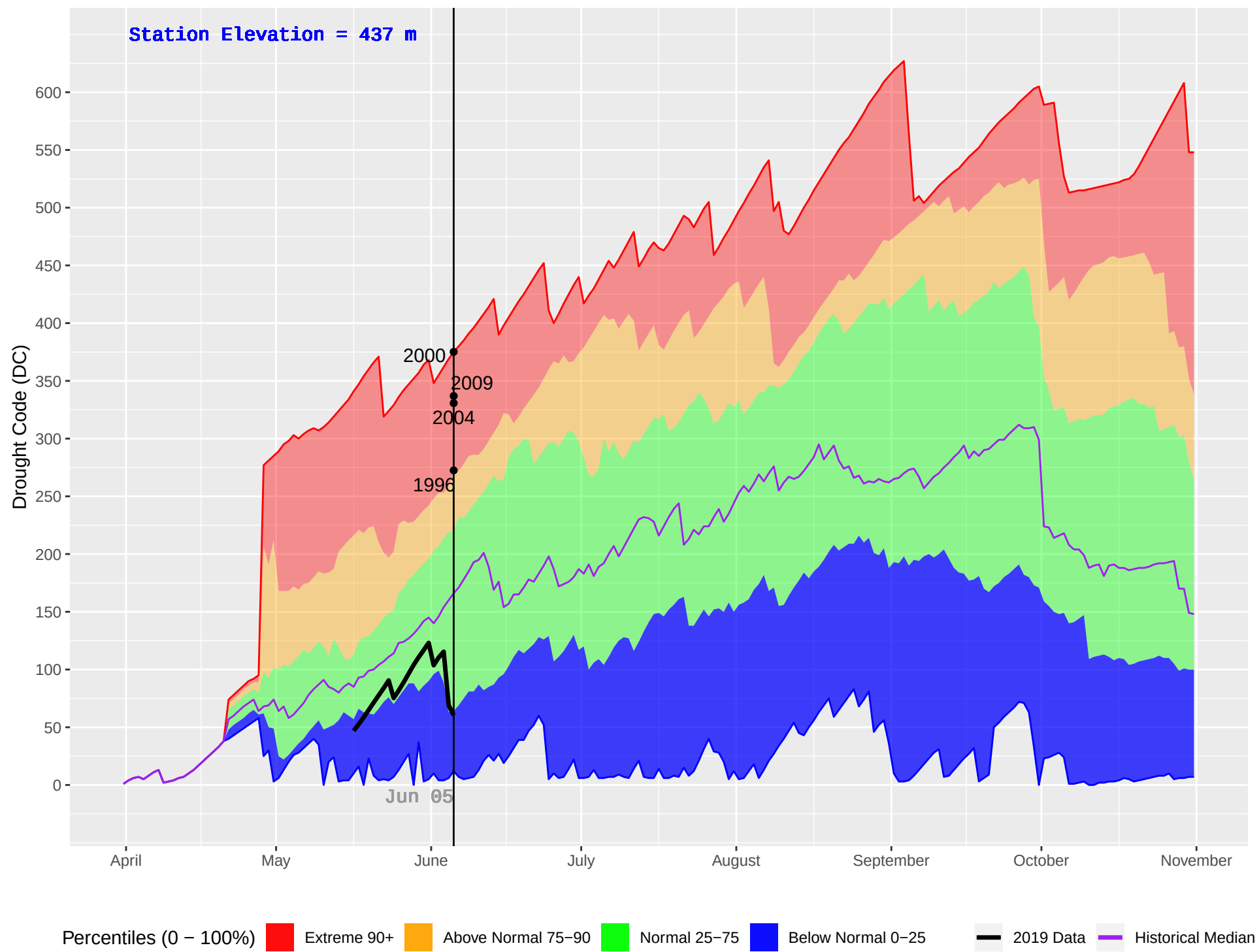
ELK MOUNTAIN (438) : Historical (1973–2018) and Current (2019) Daily Drought Code (DC)
