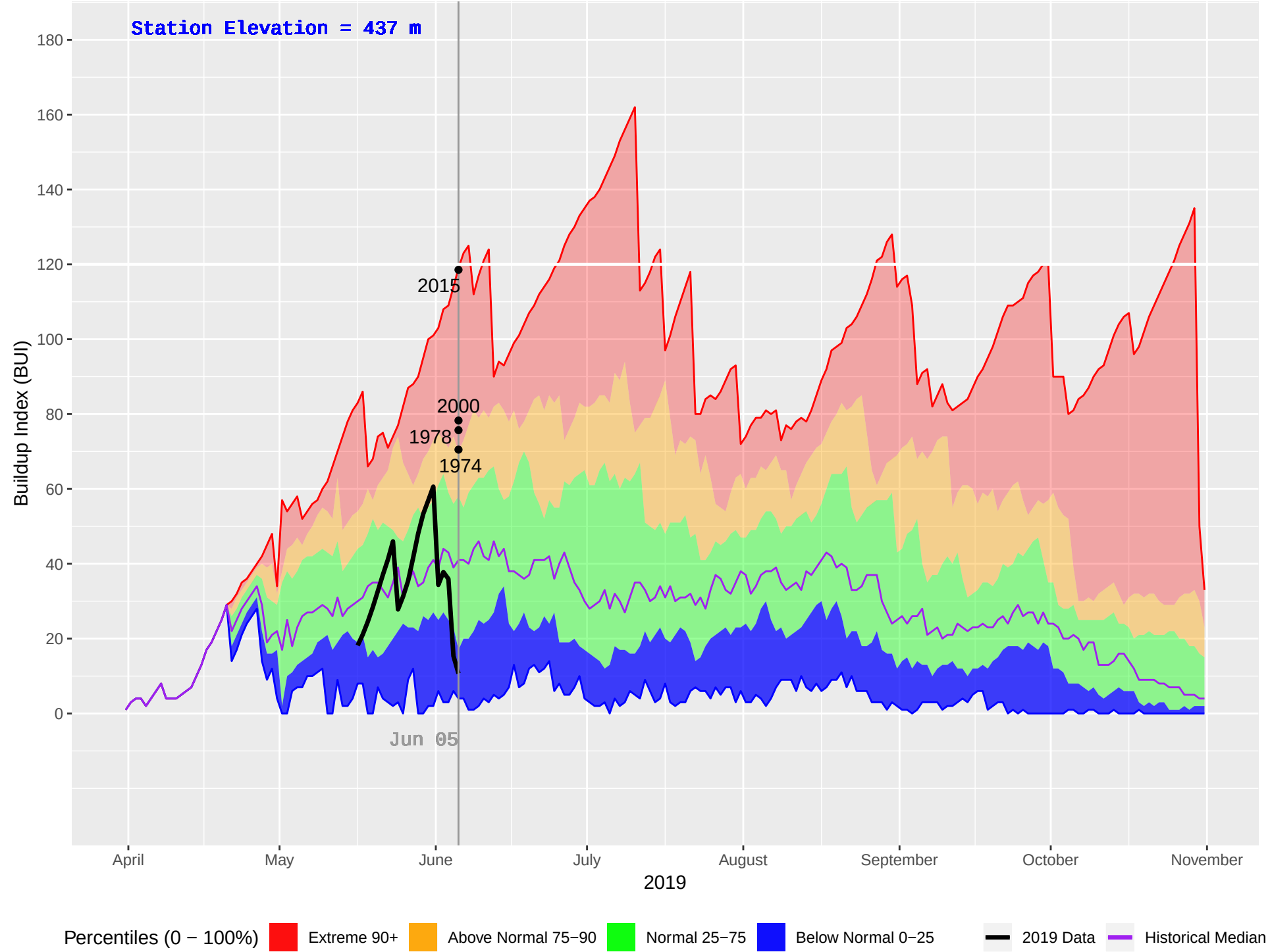
ELK MOUNTAIN (438) : Historical (1973–2018), Current (2019) Daily Buildup Index (BUI)
