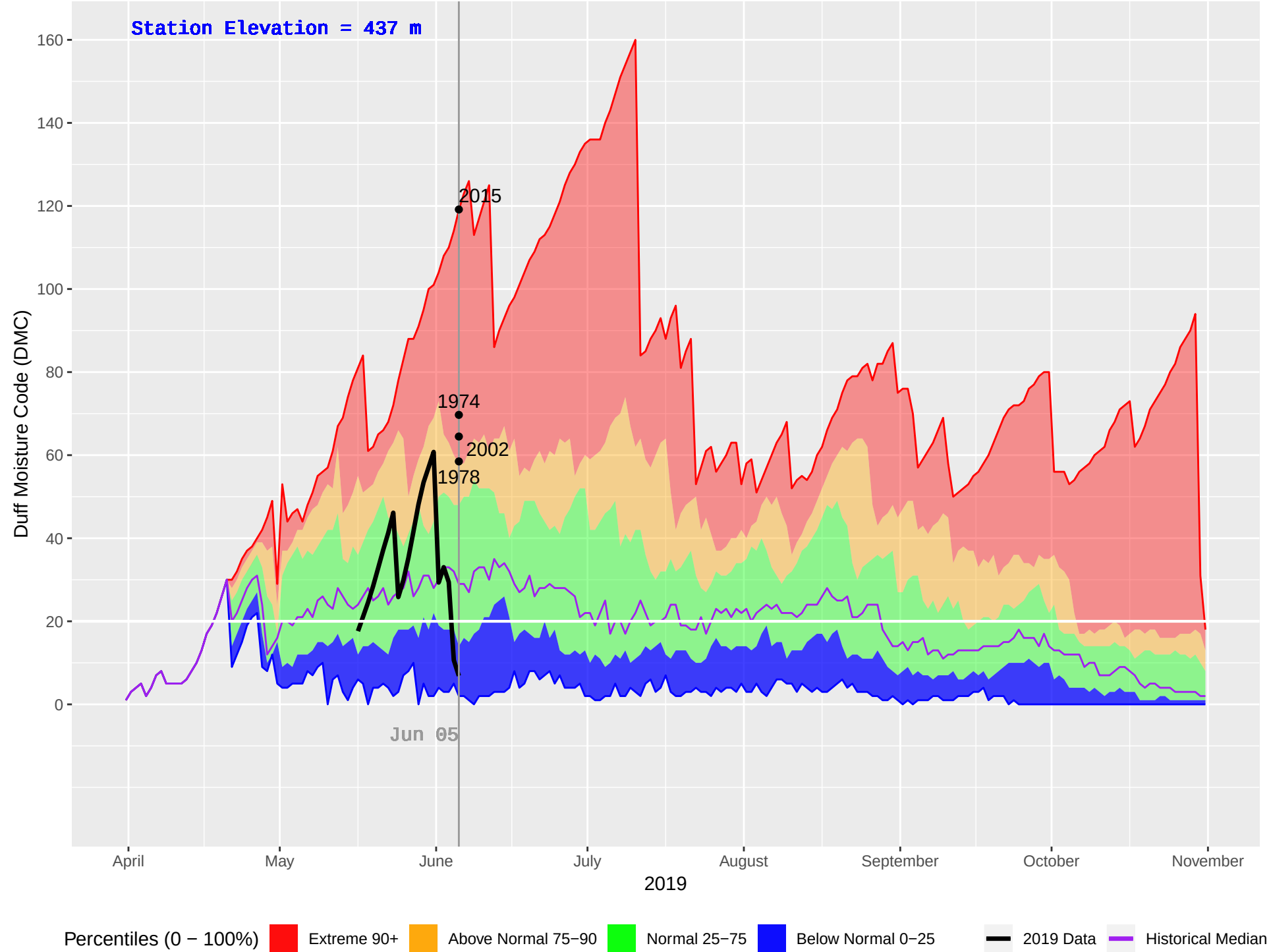
ELK MOUNTAIN (438) : Historical (1973–2018), Current (2019) Daily Duff Moisture Code (DMC)
